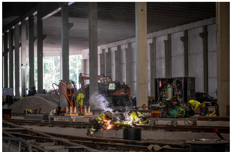
Photo: Track works at the Koskela depot site
